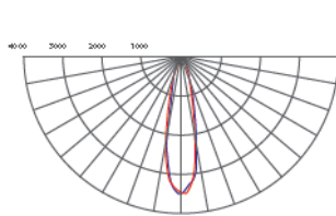
LIGHT DISTRIBUTION
