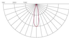
LIGHT DISTRIBUTION
