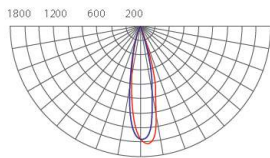
LIGHT DISTRIBUTION
