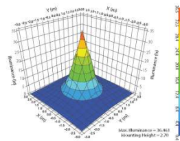
OPTICAL Characteristics
