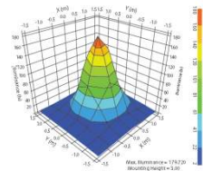
OPTICAL Characteristics
