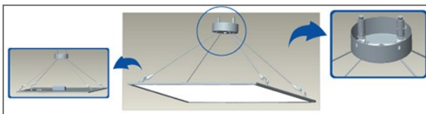
Hanging Mounting Kit: CPSURFMOUNTKIT
