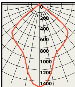
Goniogram for a 90° Fixture
