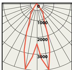
Goniogram for a 40° Fixture
