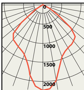
Goniogram for a 90° Fixture
