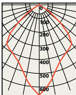
Goniogram for a 40° Fixture
