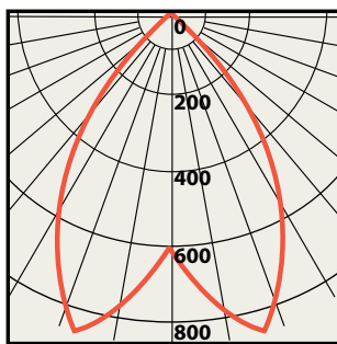
Goniogram for a 70° Fixture
