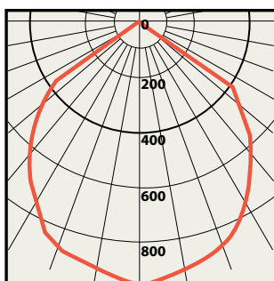
Goniogram for a 120° Fixture
