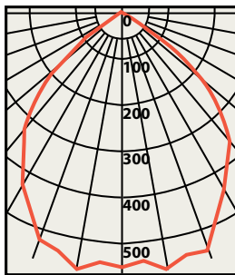
Goniogram for a 120° Fixture
